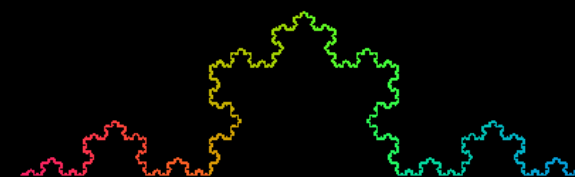
A Sierpinski triangle collapses to part of Koch Snowflake
